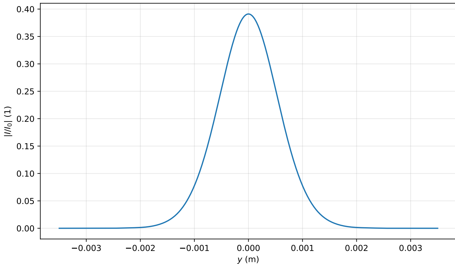
Intensity profile I(x=0, y, z=3.184)/I_0 , P_{in}=0.3P_{cr} , artificial time
